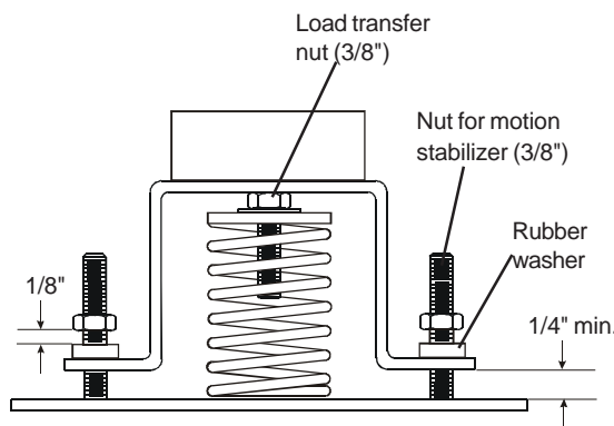
Spring Adjustment Detail
